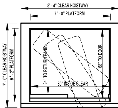
RIGHT HAND SHOWN, LEFT HAND OPPOSITE 3500 lb IN LINE
