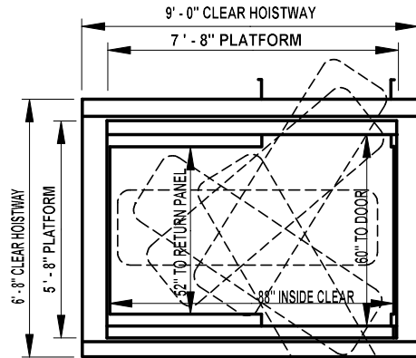
RIGHT HAND SHOWN, LEFT HAND OPPOSITE 2800 lb FRONT AND REAR
