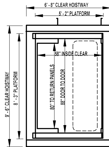
RIGHT HAND SHOWN, LEFT HAND OPPOSITE 2800 lb FRONT AND REAR
