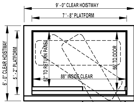
RIGHT HAND SHOWN, LEFT HAND OPPOSITE 2800 lb IN LINE
