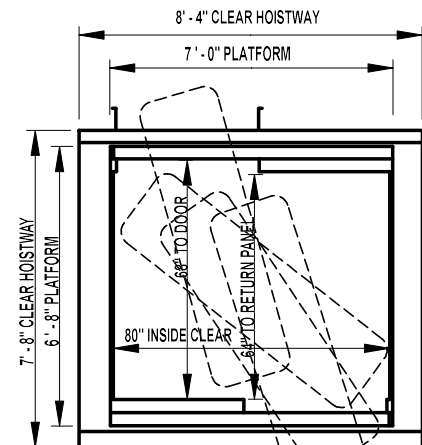
RIGHT HAND SHOWN, LEFT HAND OPPOSITE 3500 lb FRONT AND REAR
