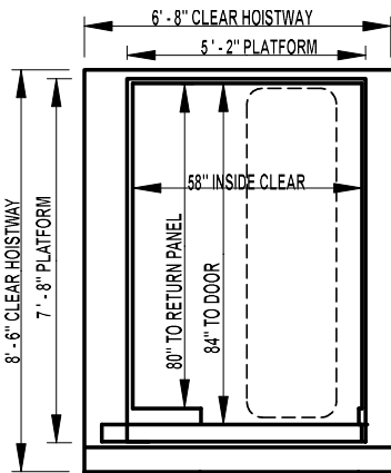
RIGHT HAND SHOWN, LEFT HAND OPPOSITE 2800 lb IN LINE
